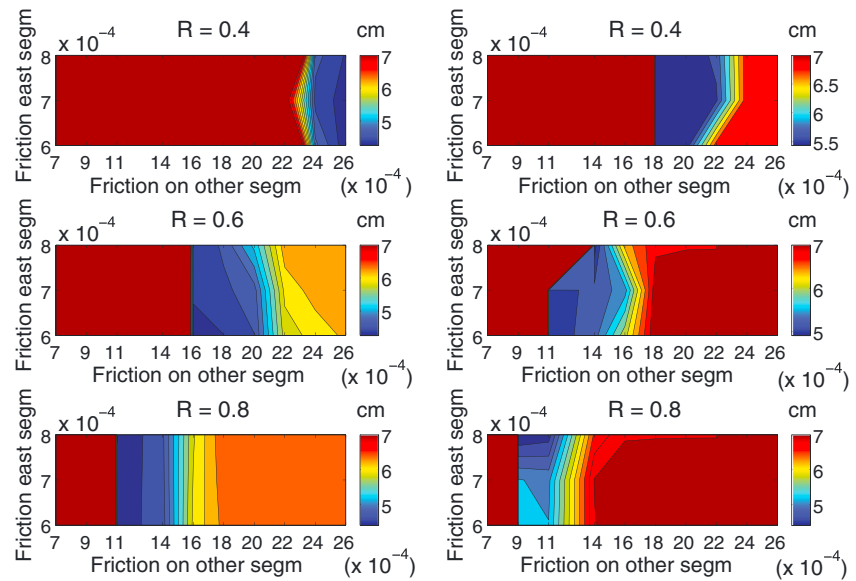
Figure 7. Variation of the WRMS misfit for the coral microatolls data set. (left column) The result for an orientation of 50^\circ and (right column) the result for an orientation of 60^\circ . The y axis is the b friction constant on the eastern Léogâne segment, and the x axis is the b friction constant on the other segments where b is the constant from equation (4).
