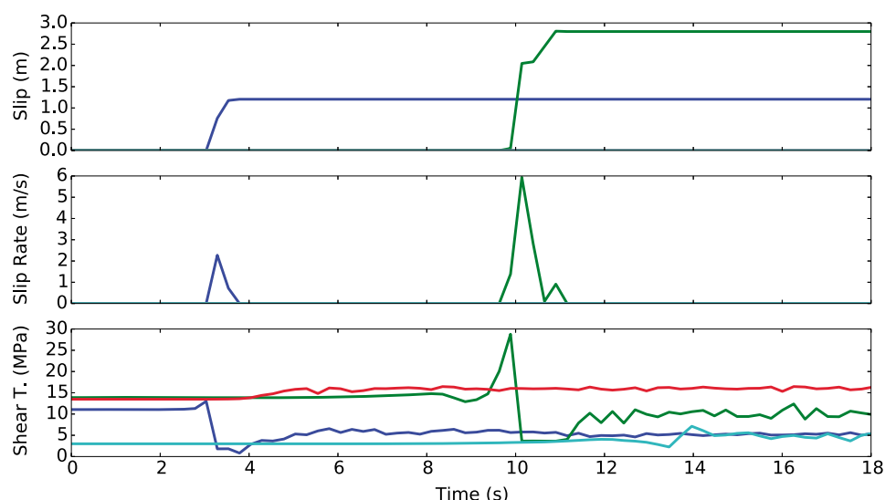
Figure 15. Slip, slip rate, and shear stress time histories for locations on the eastern Léogâne (blue line), western Léogâne (green line), Enriquillo (red line), and Trois Baies fault (cyan line) from scenario C. The location of those points are shown in Figure 2. For the point on the eastern Léogâne segment, the shear stress starts increasing at 2.8 s and slip starts at 3 s. For the corresponding point on the western Léogâne segment, slip occurs at 10 s. Although rupture does not propagate to the Enriquillo and the Trois Baies faults, significant stress change magnitude has been observed on those two faults.
